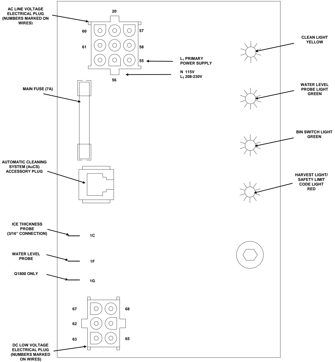
Control Board
